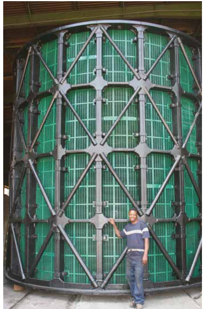
5 000 mm diameter by 5 500 mm long Trommel Screen
